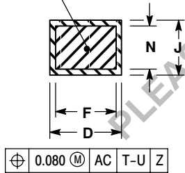
SECTION AE-AE
