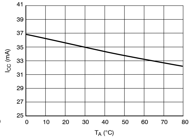
Figure 16. I_{CC} vs. T_A
