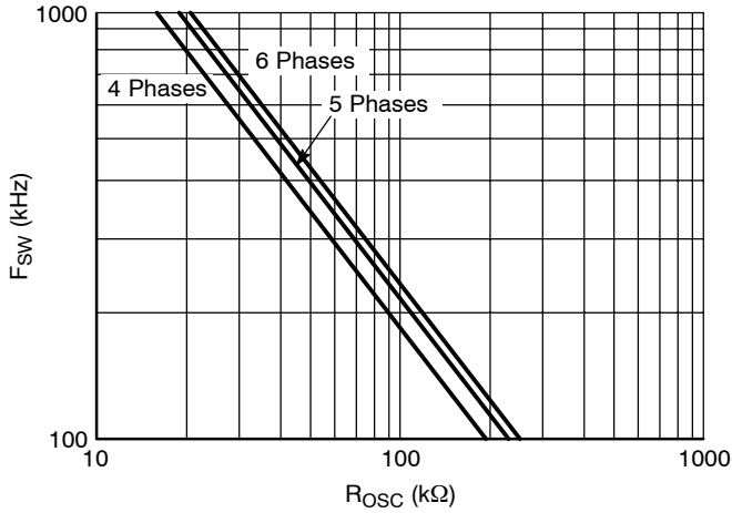
Figure 5. R_{osc} (kΩ) vs. f_{sw} (kHz)
