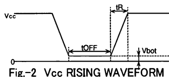
Fig.-2 Vcc RISING WAVEFORM
