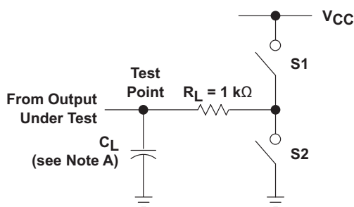
LOAD CIRCUIT
