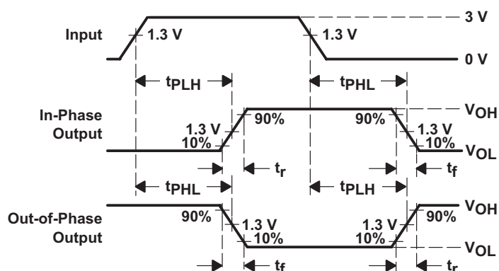
VOLTAGE WAVEFORMS
