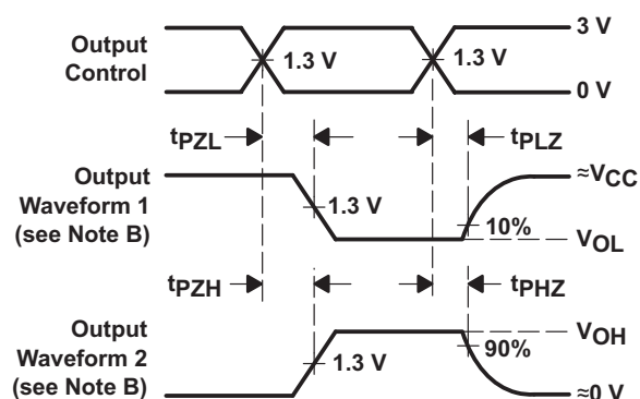
VOLTAGE WAVEFORMS
