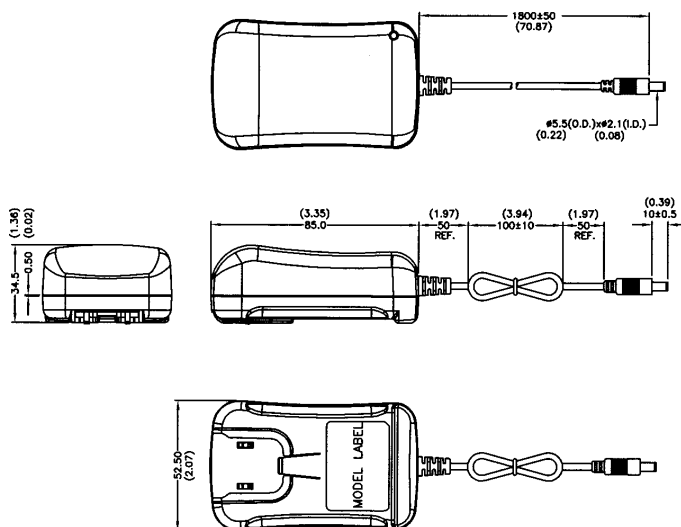
ASSEMBLY FROM HOUSING AND AUST. CLIP
