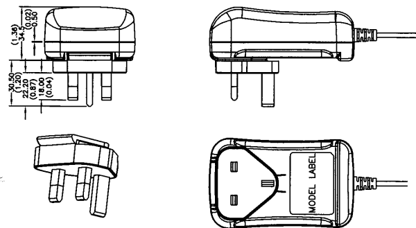
ASSEMBLY FROM HOUSING AND U.K. CLIP
