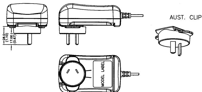
ASSEMBLY FROM HOUSING AND AUST. CLIP
