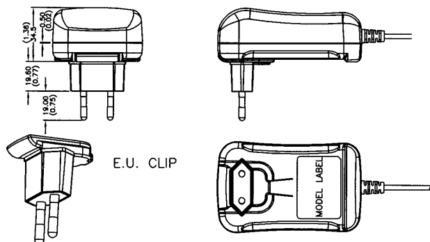
ASSEMBLY FROM HOUSING AND E.U. CLIP
