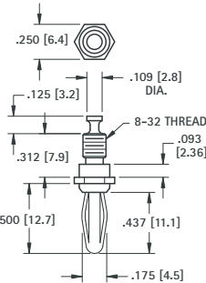
.175 (4.5) Plug
