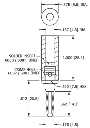
.175 (4.5) Plug
