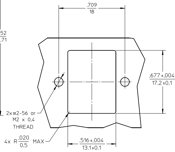
RECOMMENDED MOUNTING PATTERN SCALE 2.5:1
