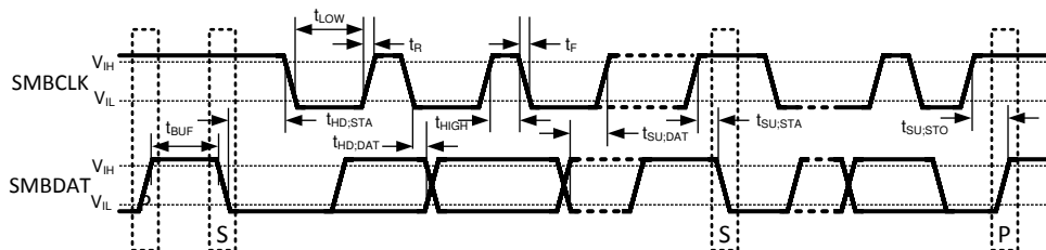
Figure 5-1. SMBus Communication
