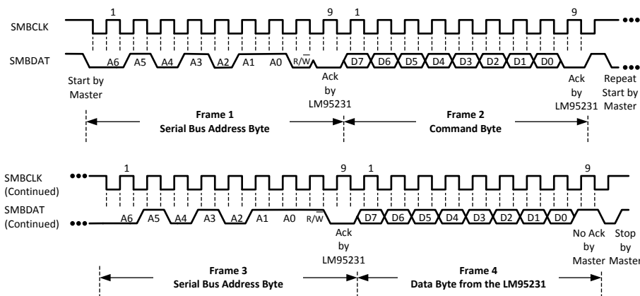
Figure 6-5. SMBus Timing Diagrams for Access of Data
