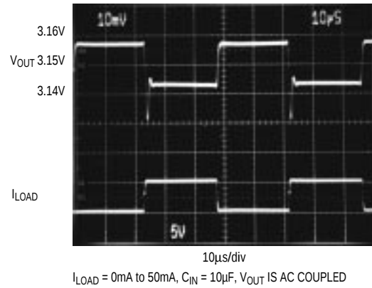
LOAD TRANSIENT
