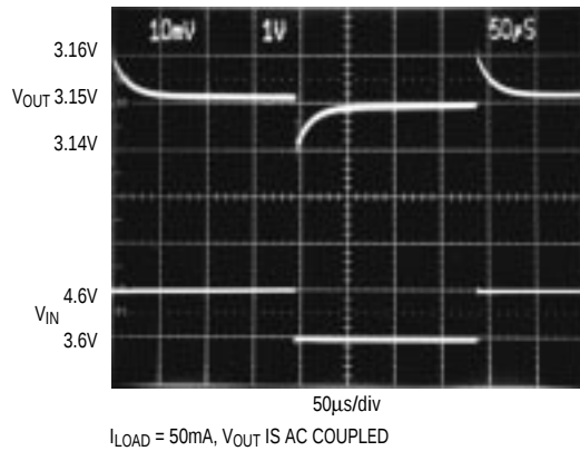
LINE TRANSIENT
