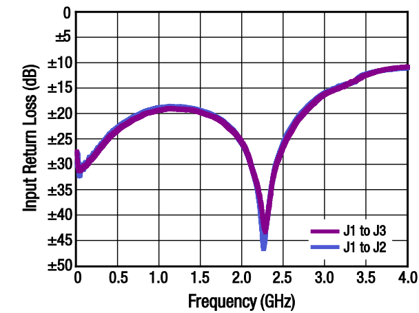
Figure 5. Input Return Loss (Insertion Loss State) vs Frequency
