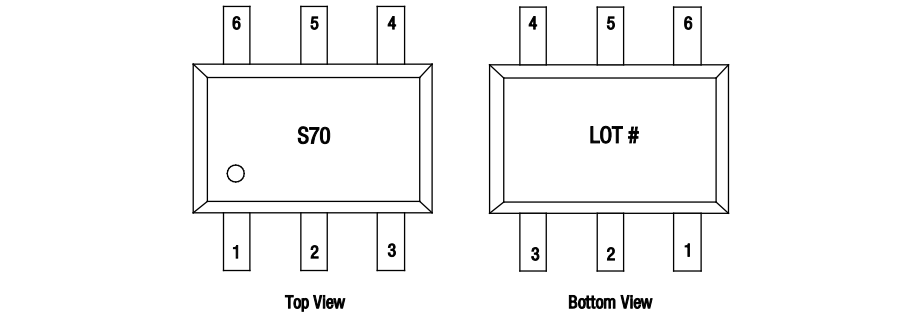
Figure 9. Typical Case Markings
