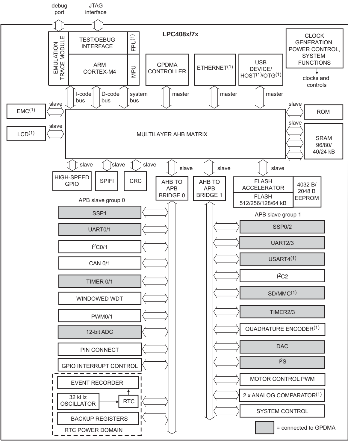
Fig 1. Block diagram
