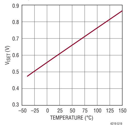
V_{ISET} vs Temperature
