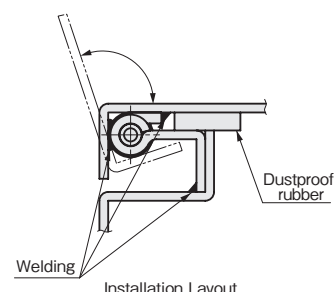
Installation Layout
