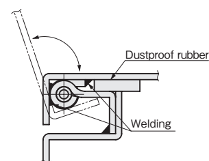
Installation Layout
