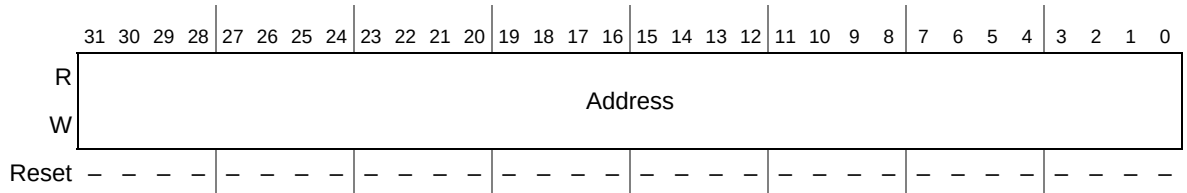
Figure 2-4. Stack Pointer Registers (A7 and OTHER_A7)
