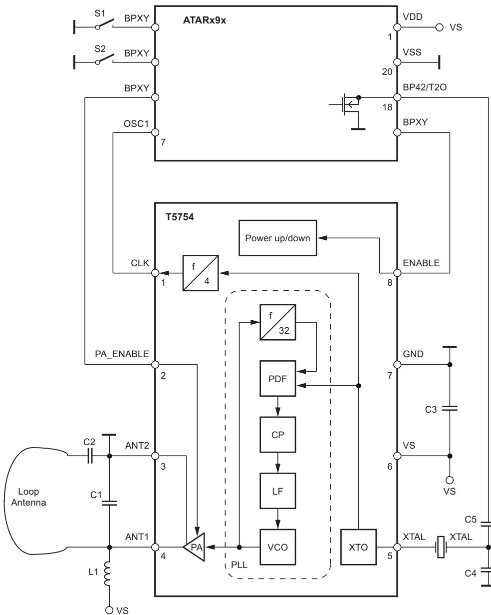
Figure 4-4. FSK Application Circuit
