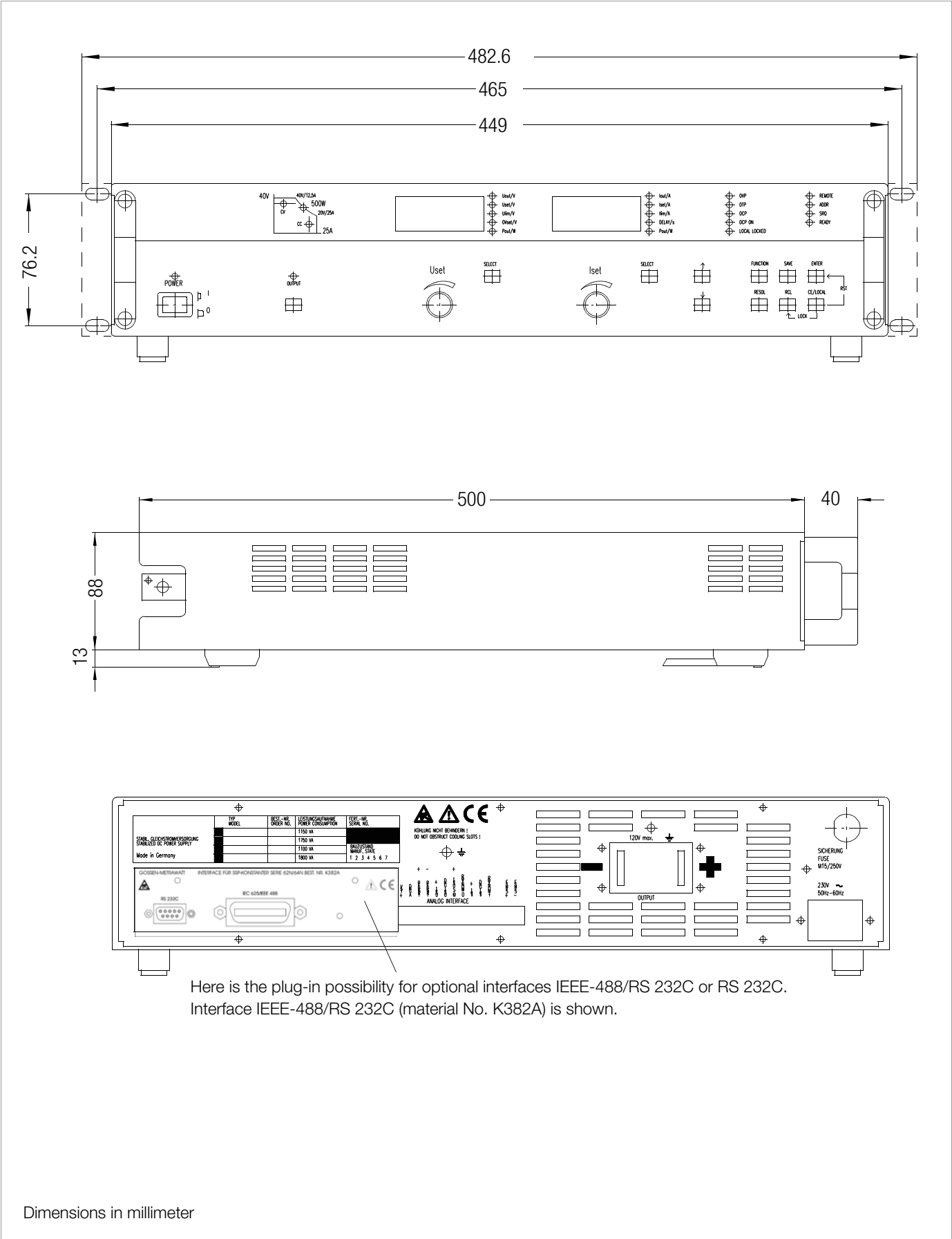
Dimensional Drawing
