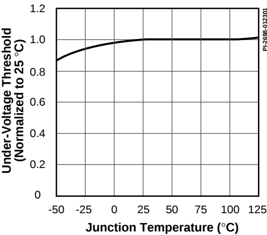
Figure 30. Undervoltage Threshold vs. Temperature.
