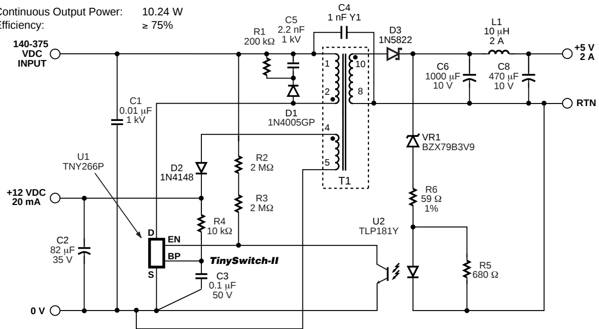
Figure 15. 10 W Standby Supply.
