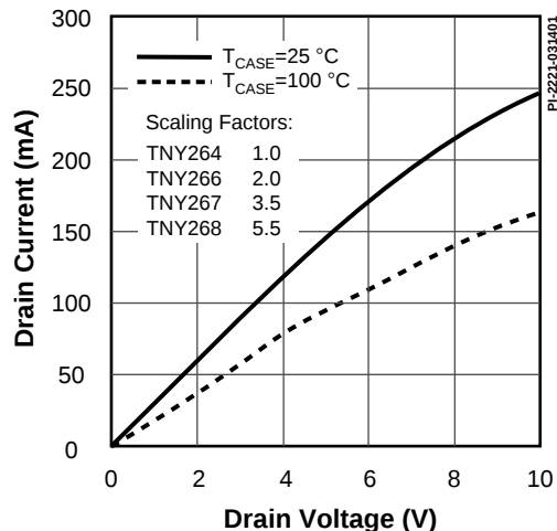
Figure 27. Output Characteristic.
