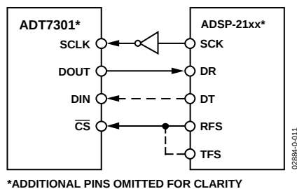
Figure 18. ADT7301-to-ADSP-21 Interface
