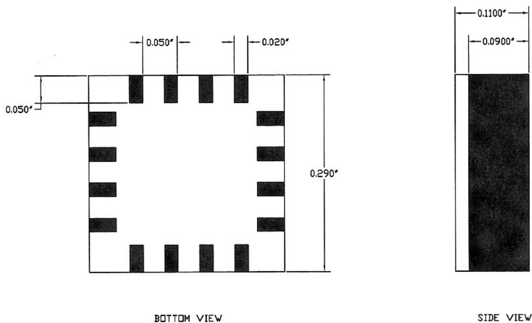
PACKAGE DRAWING HMC1053 (16-PIN LCC)
