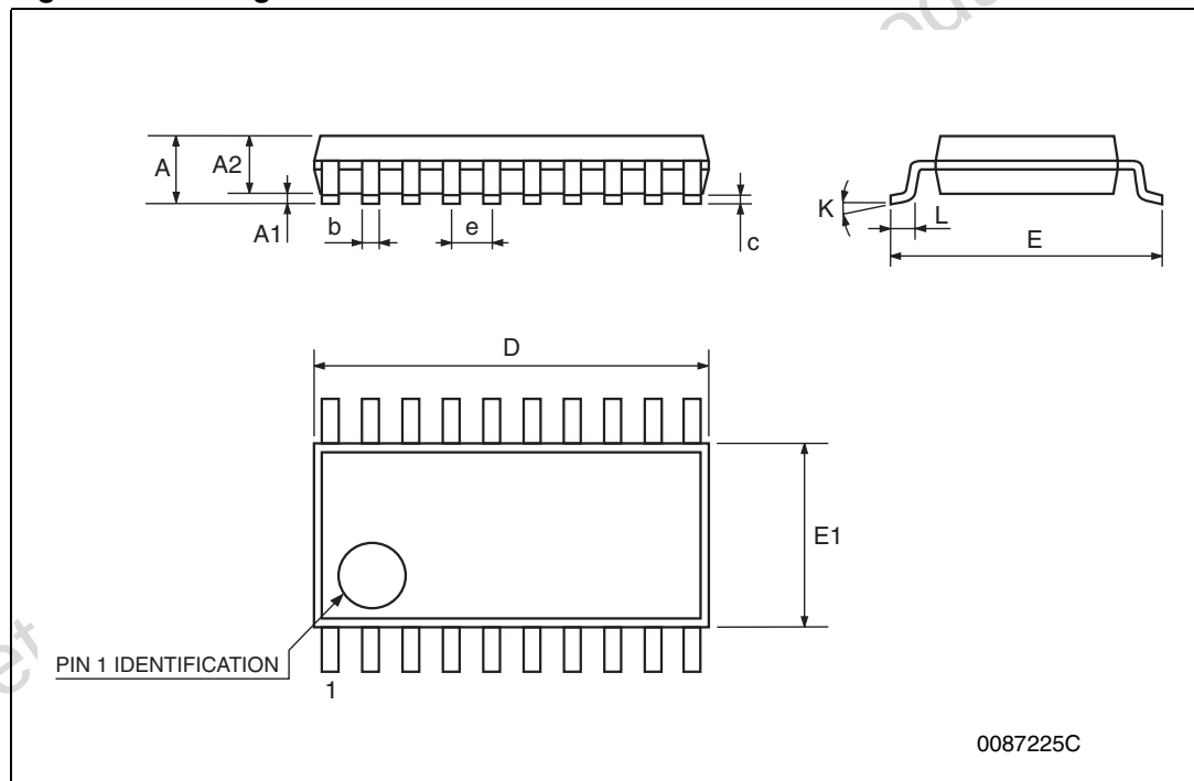
Figure 6. Package dimensions
