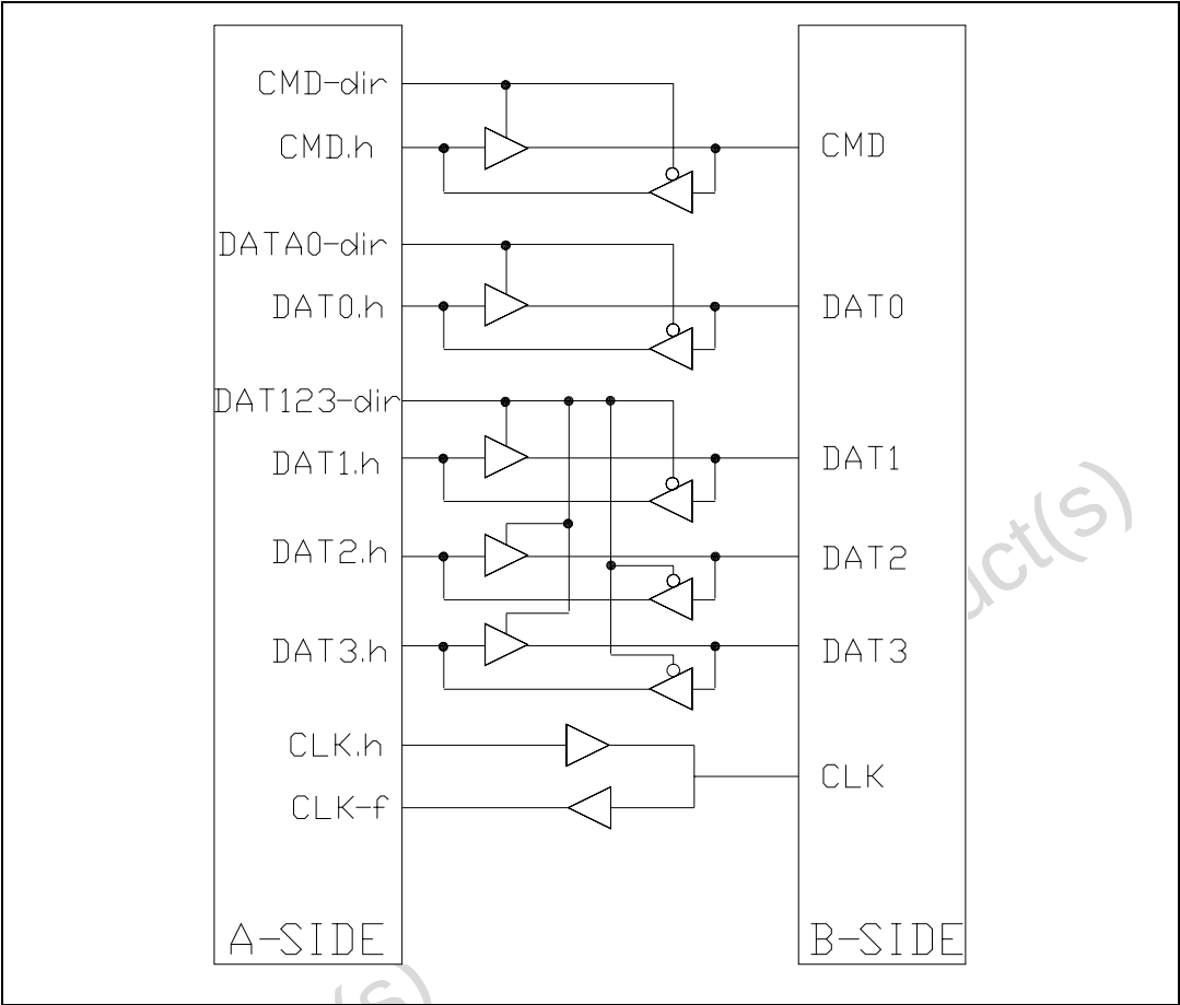
Figure 1. Logic diagram
