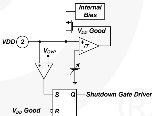
Figure 21. Internal OVP Block
