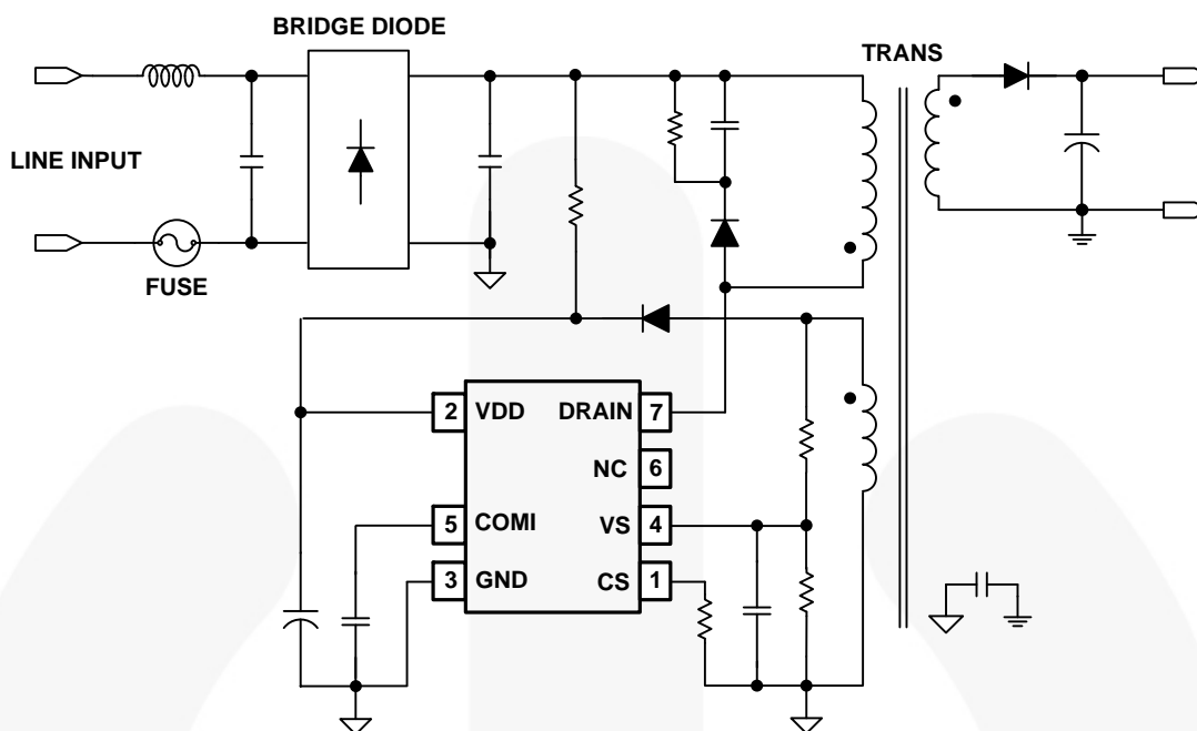
Figure 1. Typical Application
