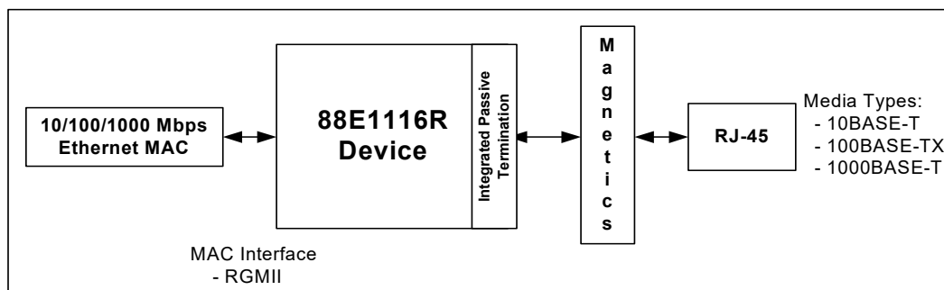
88E1116R Device used in Copper Application
