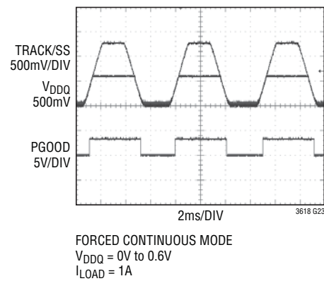
Tracking Up/Down
