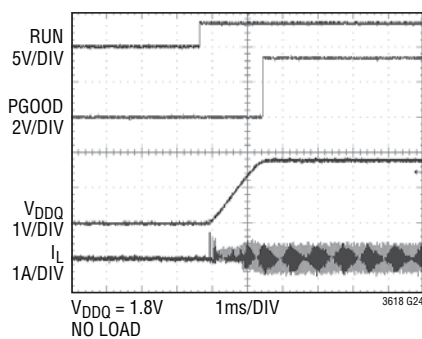
Internal Start-Up V_{DDQ}
