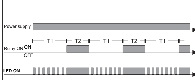
Function Ab - Asymmetrical Recycler - OFF first
