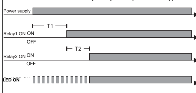
Function Dt - Two state Delay on operate (2xSPDT only)
