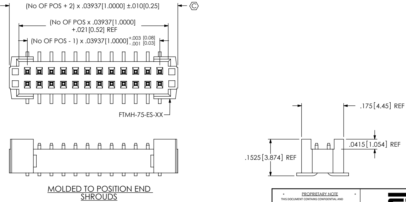
FIG 2 -ES: END SHROUDS FTMH-112-02-X-DV-ES SHOWN (DIFFERENT AS SHOWN, OTHERWISE SAME AS FIG 1)
