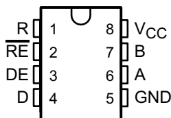
SN65176B D OR P PACKAGE SN75176B D, P, OR PS PACKAGE (TOP VIEW)
