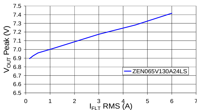
V_{OUT} Peak vs. I_{FLT} ( I_{out}=0 )
