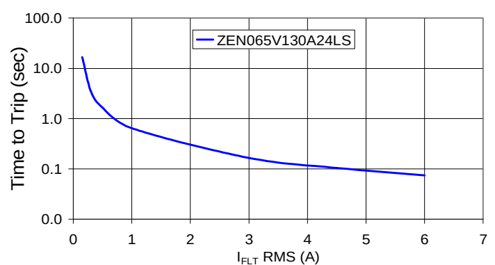
Time to Trip vs. I_{FLT} RMS ( I_{out}=0 )
