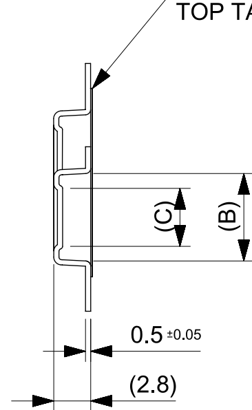
SECT. X-X
