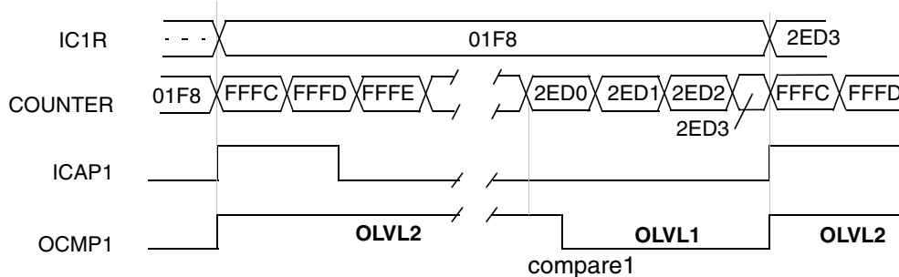
Figure 44. One Pulse Mode Timing Example
