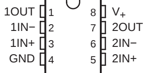
TLV342 D (SOIC) OR DGK (MSOP) PACKAGE (TOP VIEW)
