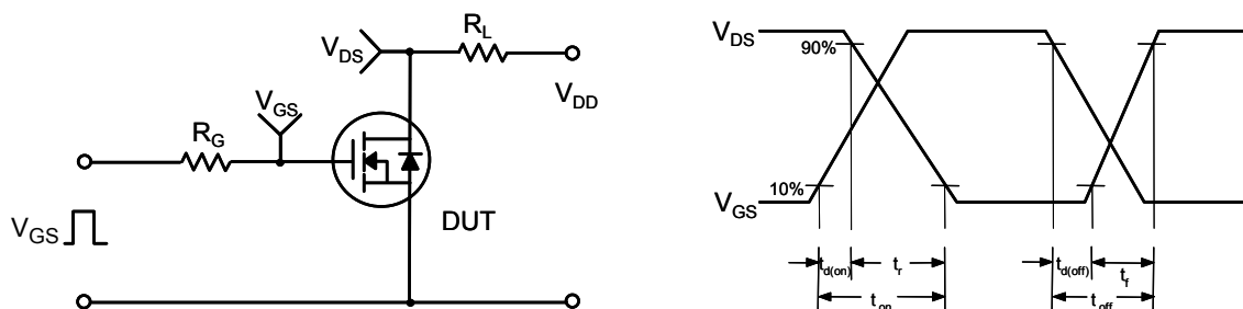
Figure 20. Resistive Switching Test Circuit & Waveforms
