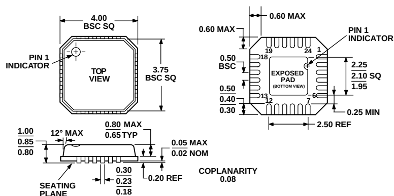
Figure 34. 24-Lead Lead Frame Chip Scale Package [LFCS]
