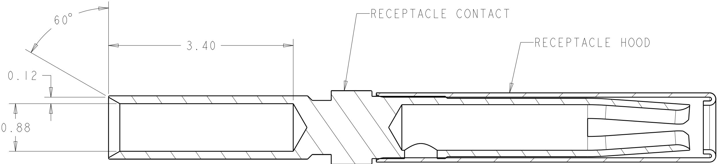
SECTION Z-Z
