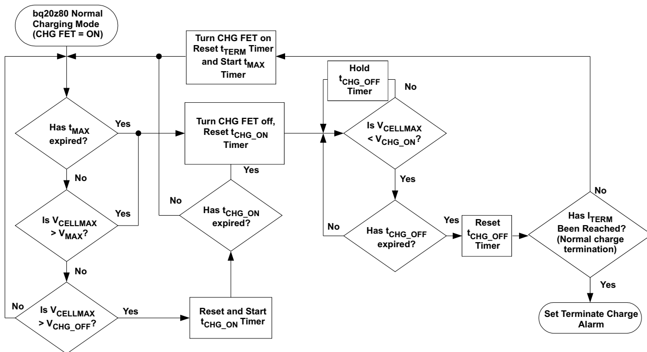
Figure 3. Pulse Charging
