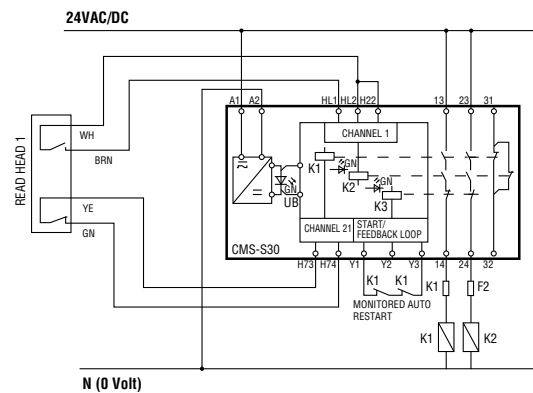
CM-S30 Application Diagram (Cat 4)
