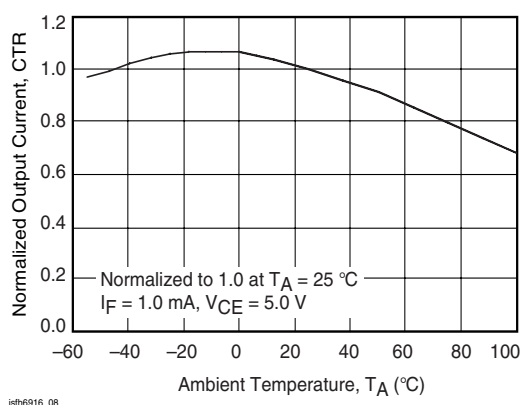
Fig. 8 Normalized Output Current vs. Ambient Temperature
