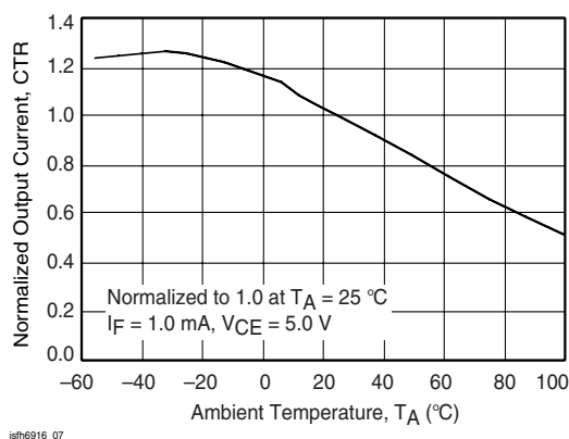
Fig. 7 Normalized Output Current vs. Ambient Temperature
