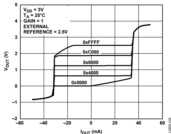
Figure 30. Source and Sink Capability at 3 V
