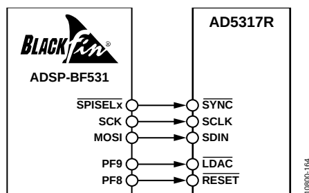
Figure 51. ADSP-BF531 Interface
