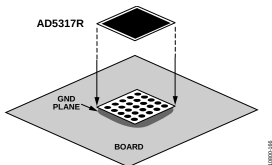
Figure 53. Pad Connection to Board
