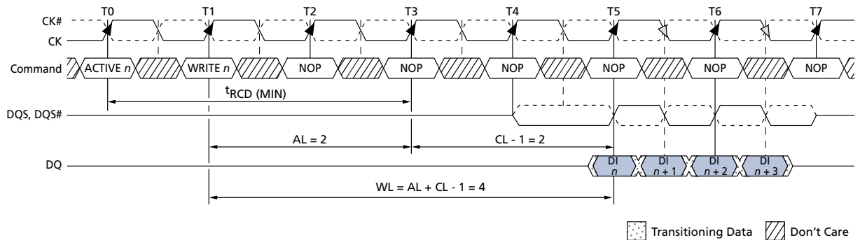
Figure 39: WRITE Latency
