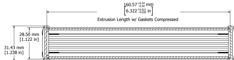
SECTION Y-Y
