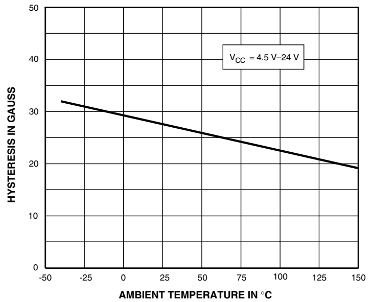
HYSTERESIS
