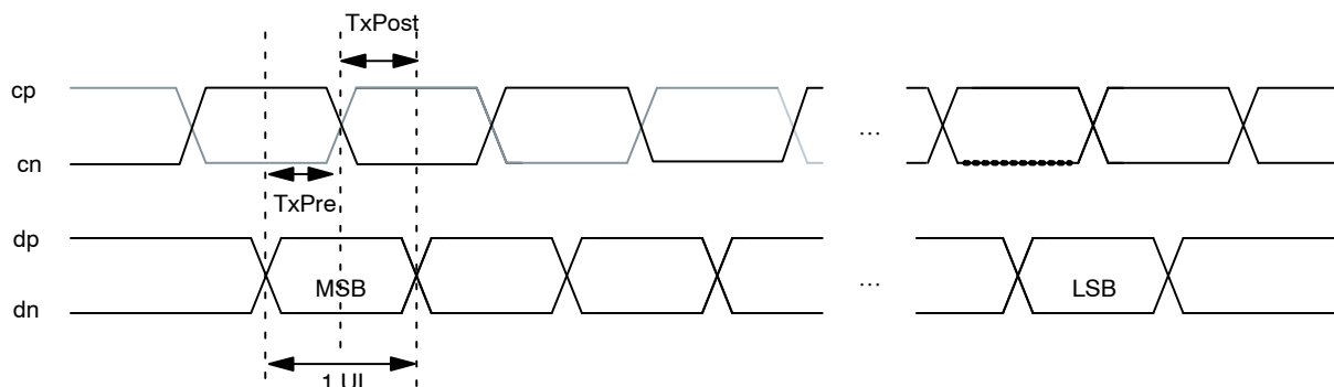
Figure 8. Timing Diagram
