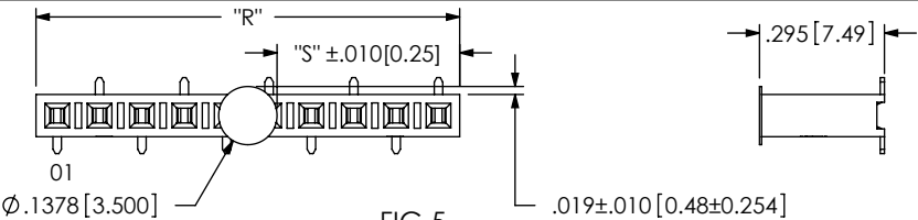
FIG 5 -K: KAPTON PAD (SSM-110-XXX-SV-K SHOWN) (DIFFERENT AS SHOWN, OTHERWISE SAME AS FIG 1) "R" = SEE FIG 1, SHEET 1 FOR OAL "S" = "R"/2 - .0689 [1.750]
