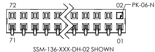
FIG 7 POLARIZATION (DIFFERENT AS SHOWN, OTHERWISE SAME AS FIG 1)
