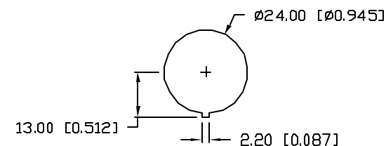
PANEL CUTOUT
