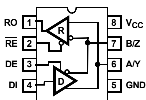
ISL32601E, ISL32603E (8 LD MSOP, SOIC) TOP VIEW
