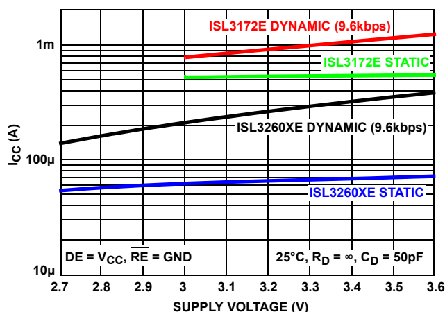
FIGURE 1. ISL32600E AND ISL32601E HAVE A 9.6\text{kbps} OPERATING I_{CC} LOWER THAN THE STATIC I_{CC} OF MANY EXISTING 3\text{V} TRANSCEIVERS
