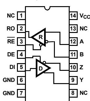
ISL32600E, ISL32602E (14 LD SOIC) TOP VIEW
