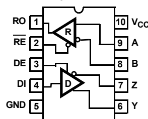
ISL32600E, ISL32602E (10 LD MSOP) TOP VIEW
