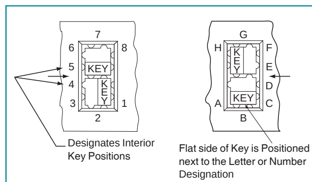
KEY LOCATIONS DAUGHTER BOARD OR INPUT/OUTPUT CONNECTORS
