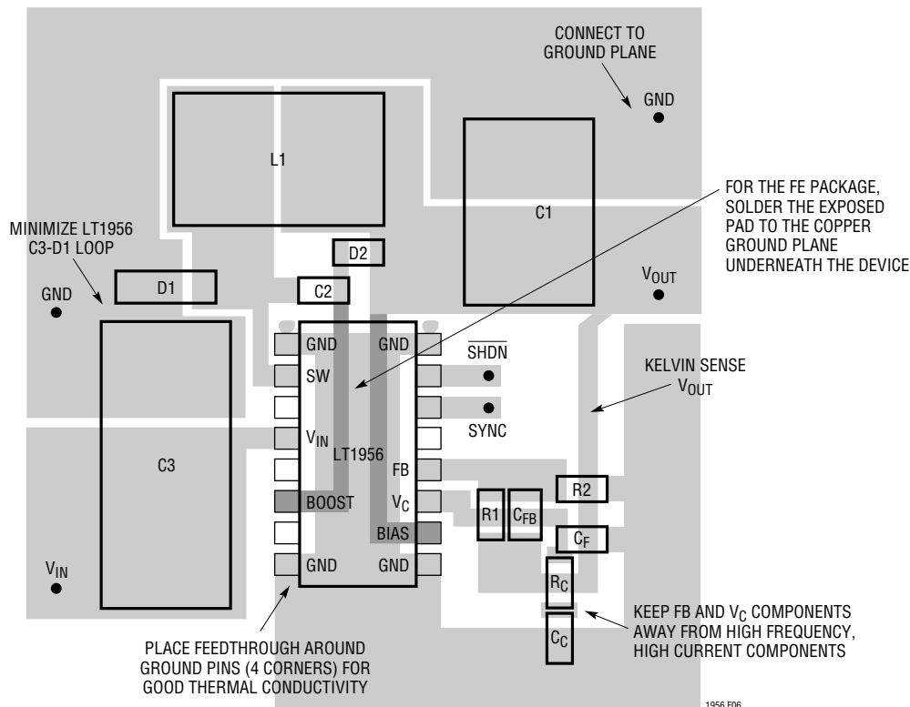
Figure 6. Suggested Layout
