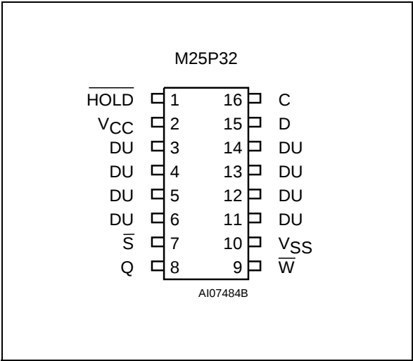
Figure 4. SO Connections
