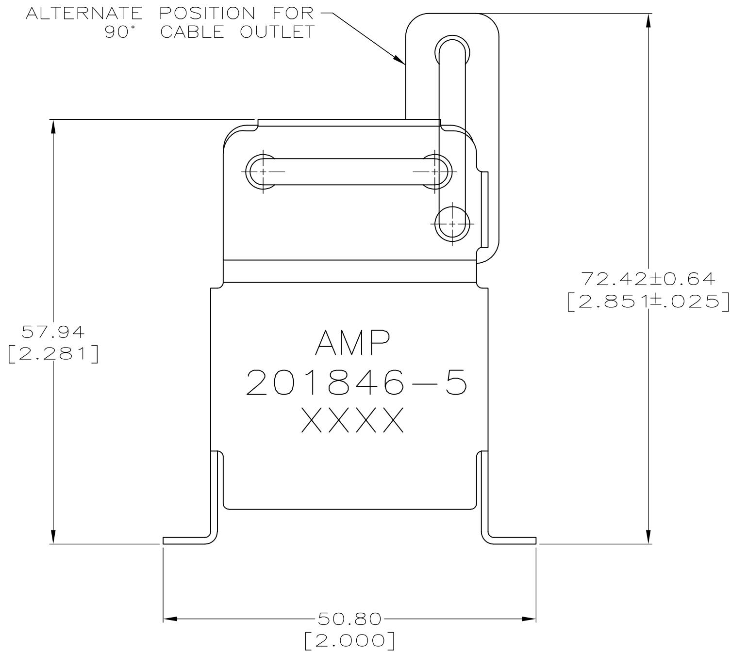
ASSEMBLED VIEW
