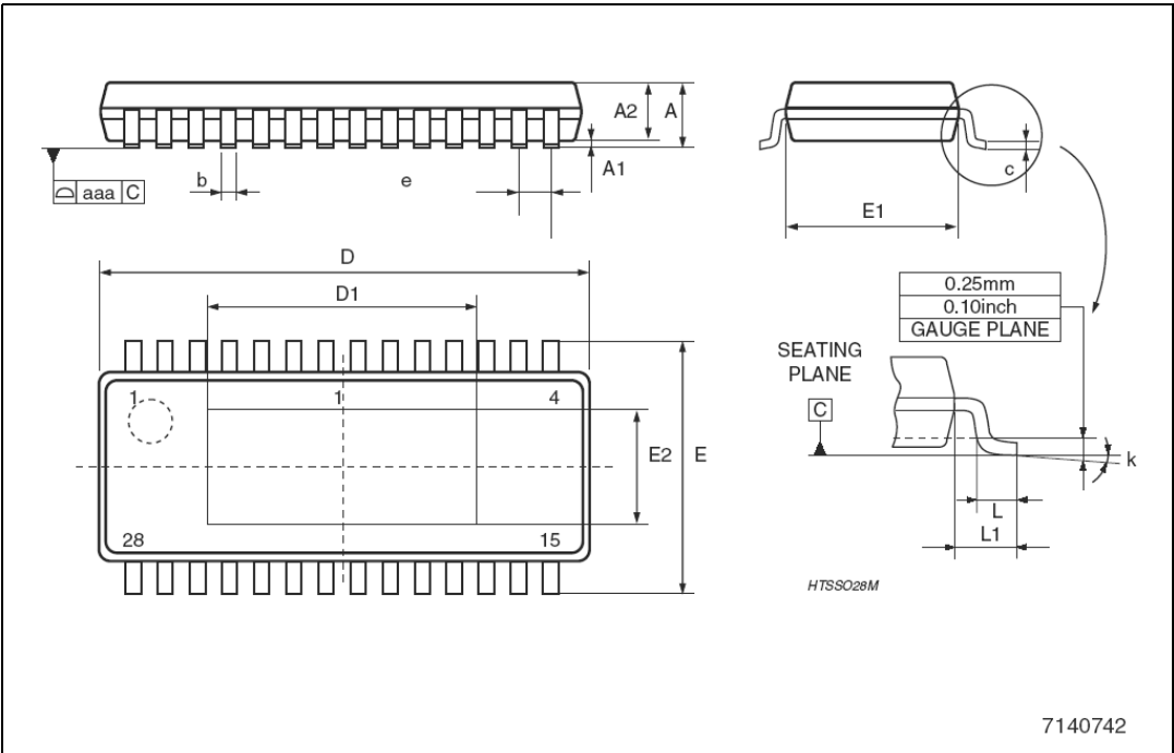
Figure 26. Package dimensions
