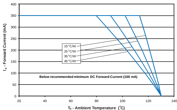
Figure 18. Maximum forward current vs. ambient temperature, based on T_{JMAX} = 130^{\circ}\text{C} , PC amber LXM2-PL01 emitters.
