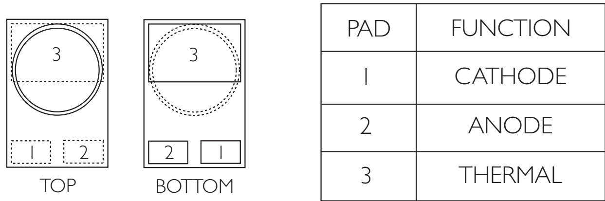
Figure 3. Pad configuration.
