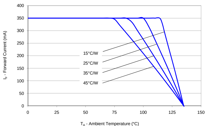
Figure 16. Maximum forward current vs. ambient temperature, based on T_{JMAX} = 135^{\circ}\text{C} , red LXML-PD01, red-orange LXML-PH01 & amber LXML-PL01 emitters.
