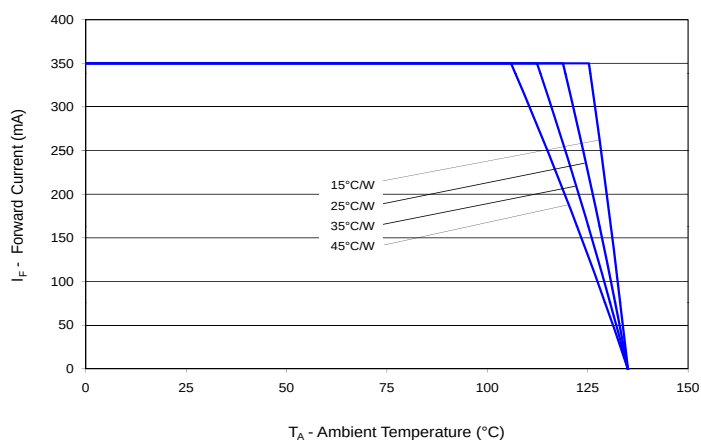
Figure 17. Maximum forward current vs. ambient temperature, based on T_{JMAX} = 135^{\circ}\text{C} , red LXM2-PD01, deep red LXM3-PD01 & red-orange LXM2-PH01 emitters.
