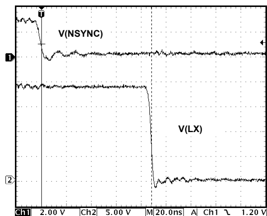
FIGURE 15. NSYNC TO LX SYNCHRONIZATION DELAY
